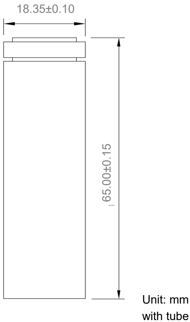
Fig. 1. Outline Dimensions of INR18650/25P
